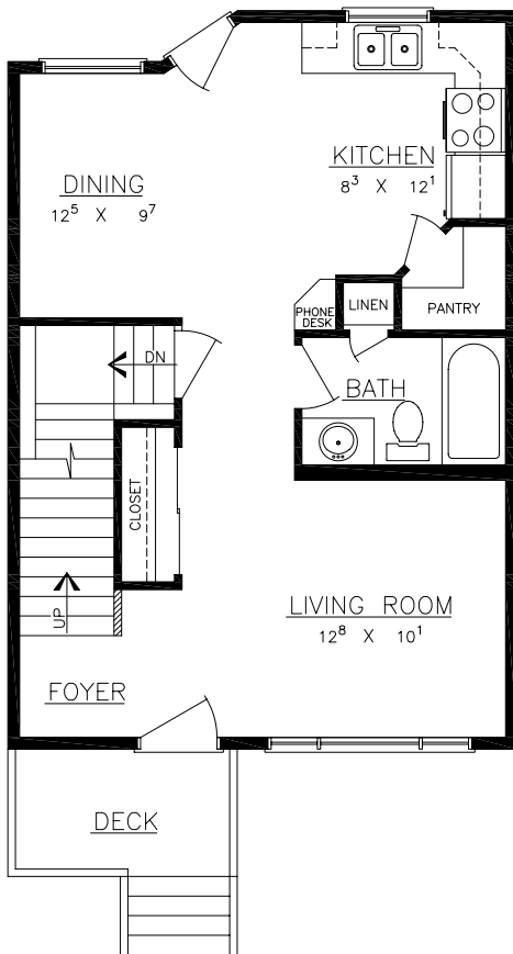
MAIN FLOOR PLAN AREA = 564 S.F.
